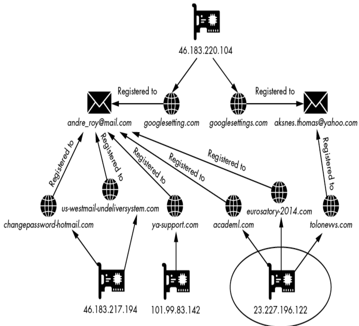
Figure 8-18: Diagram showing the IP address and name similarities between both registrant addresses created with Maltego
