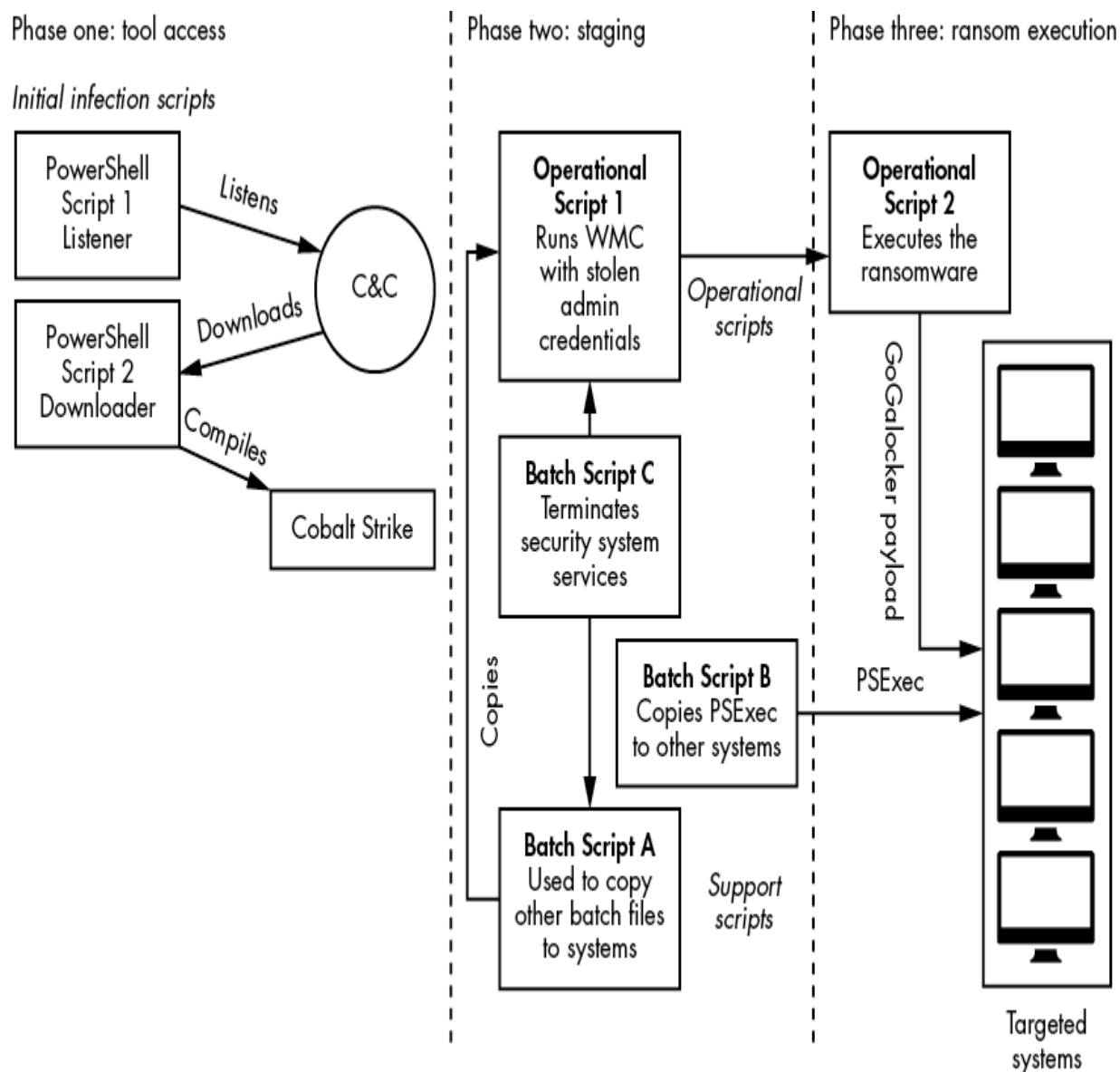
Figure 3-1: Stages of the GoGalocker compromise
