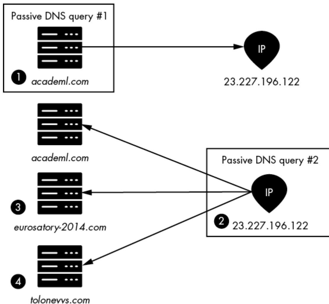
Figure 8-16: Passive DNS results for the domain academl.com and IP address 23.227.196.122
