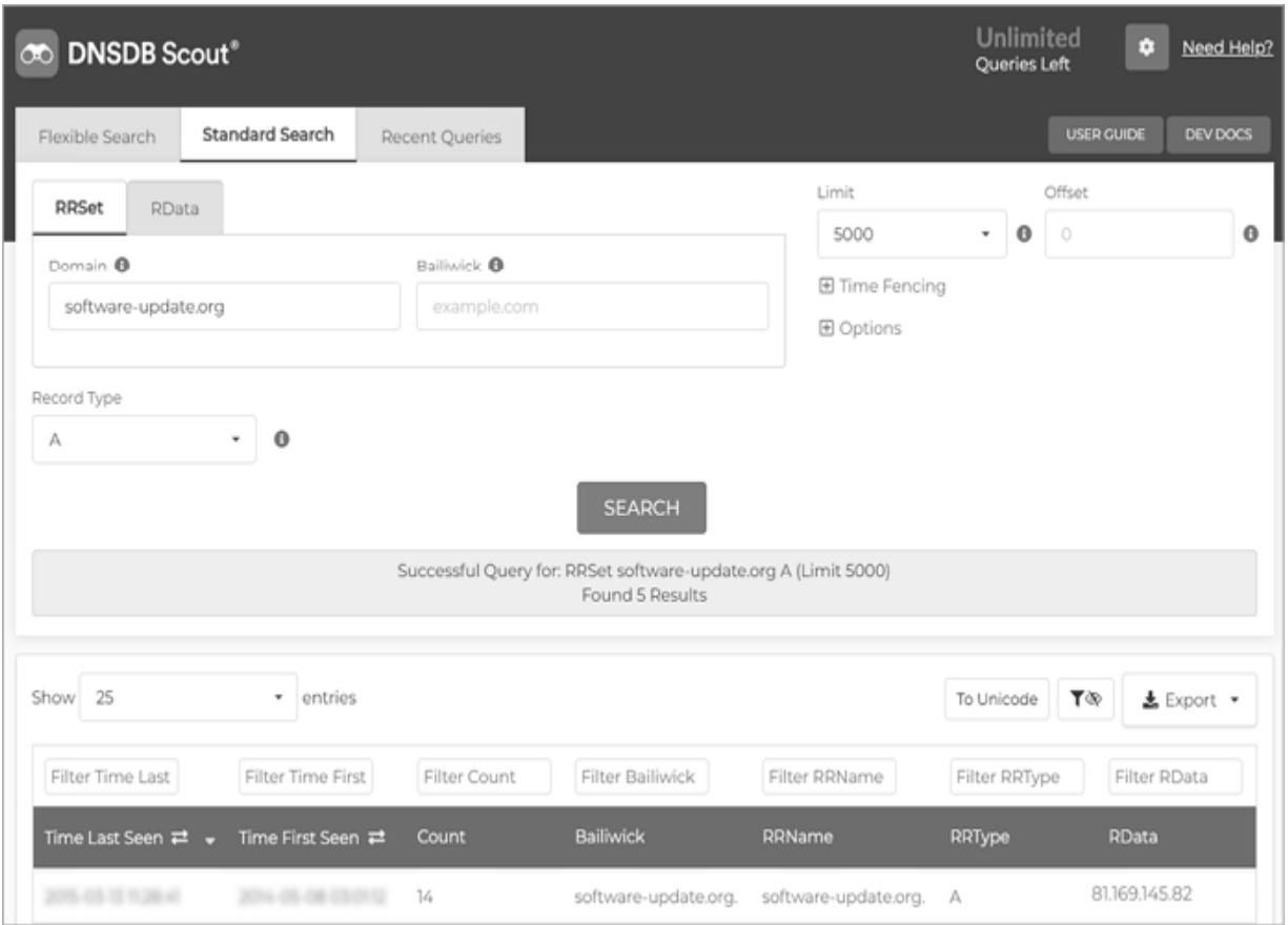
Figure 8-15: Passive DNS results for software-update.org obtained from Farsight DNSDB 12
